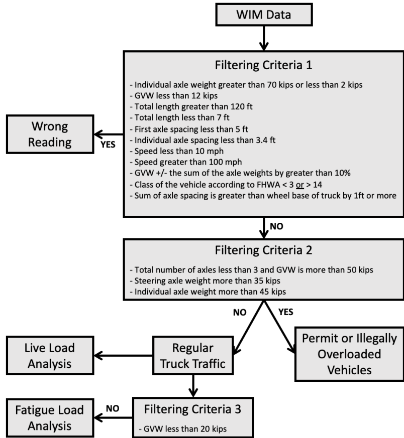
Figure 1: NCHRP 12-83 Filter (Wassef et al, 2014)
