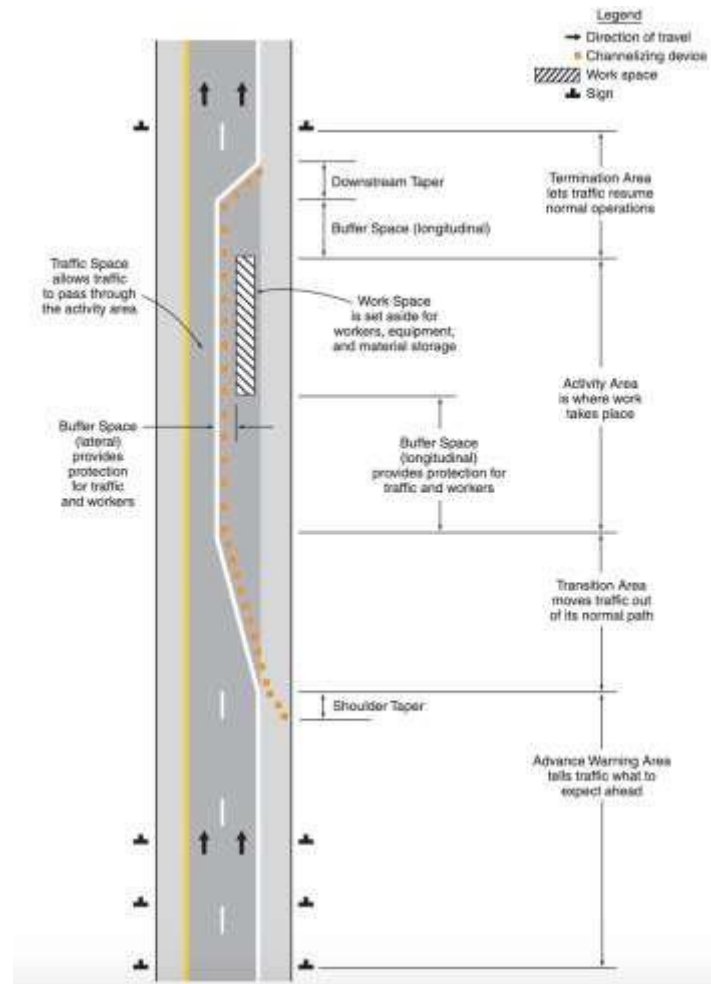
Figure 1 Temporary Traffic Control Zone as defined by the MUTCD (69)
